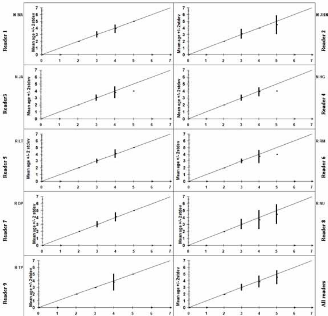
Figure 10. Norwegian otoliths from winter 2006 age bias plots. The mean age recorded +/- 2stdev of each age reader and all readers combined are plotted against the MODAL age. The estimated mean age corresponds to MODAL age, if the estimated mean age is on the 1:1 equilibrium line (solid line). RELATIVE bias is the age difference between estimated mean age and MODAL age.
