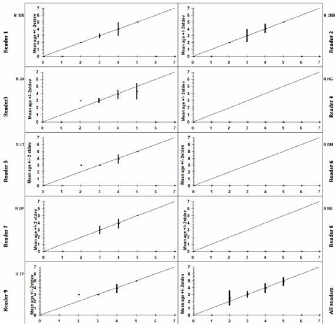
Figure 6. Russian otoliths from winter 2005 age bias plots. The mean age recorded +/- 2stdev of each age reader and all readers combined are plotted against the MODAL age. The estimated mean age corresponds to MODAL age, if the estimated mean age is on the 1:1 equilibrium line (solid line). RELATIVE bias is the age difference between estimated mean age and MODAL age.
