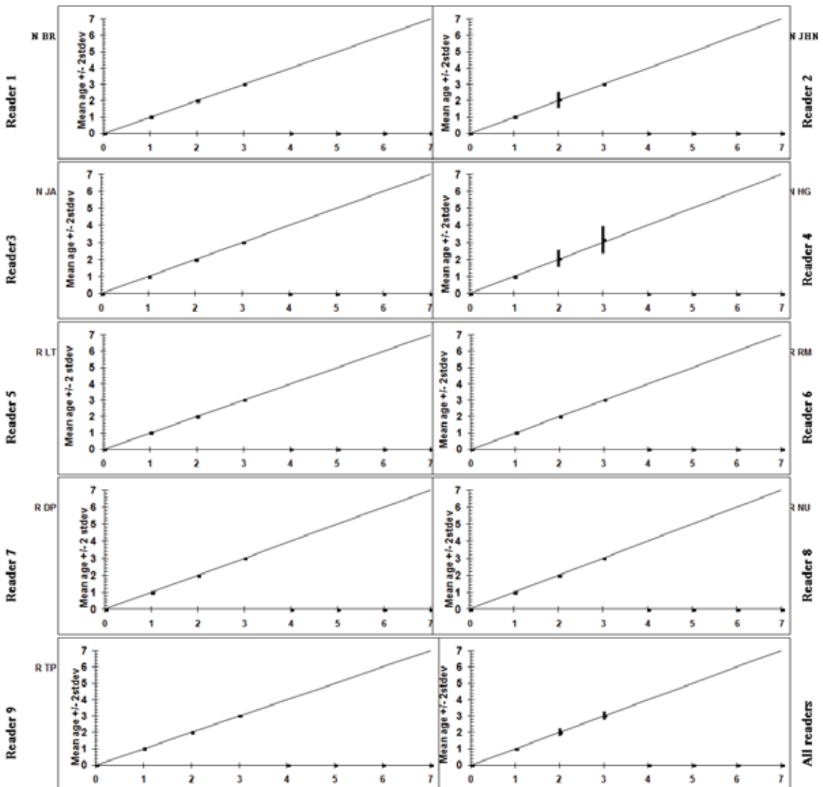
Figure 12. Russian otoliths from autumn 2006 age bias plots. The mean age recorded +/- 2stdev of each age reader and all readers combined are plotted against the MODAL age. The estimated mean age corresponds to MODAL age, if the estimated mean age is on the 1:1 equilibrium line (solid line). RELATIVE bias is the age difference between estimated mean age and MODAL age.
