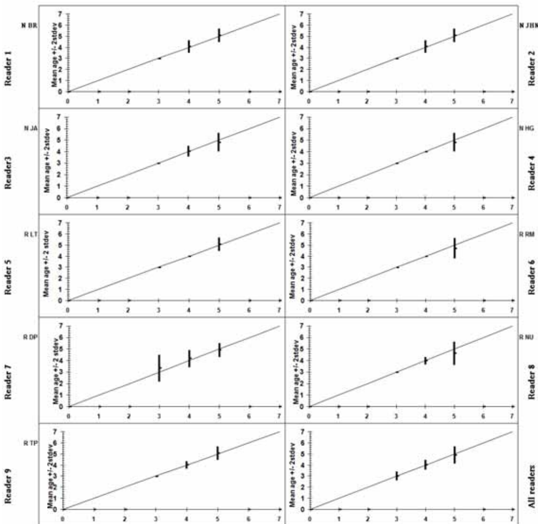
Figure 2. Norwegian otoliths from winter 2004 age bias plots. The mean age recorded +/- 2stdev of each age reader and all readers combined are plotted against the MODAL age. The estimated mean age corresponds to MODAL age, if the estimated mean age is on the 1:1 equilibrium line (solid line). RELATIVE bias is the age difference between estimated mean age and MODAL age.
