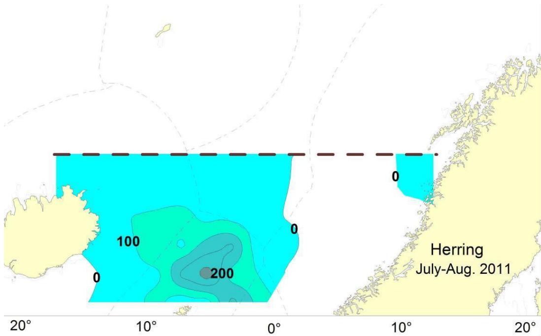
Figure 21. Contours of S_A /Nautical Area Scattering Coefficient (NASC) values of herring along the cruise track, 18 July -31 August 2011. Due to lack of coverage only data south of 66°N are included.
