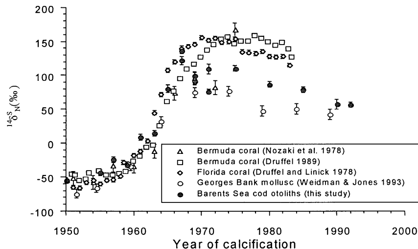
Figure 5 Comparison of several ^{14}\text{C} series developed for the subtropical, tropical, and temperate North Atlantic on the basis of corals, molluscs and cod otoliths
