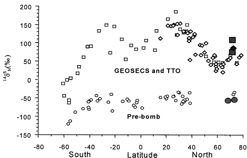
Figure 4 ^{14}\text{C} data ( ^{14}\delta^{13}\text{C} ) in surface seawater DIC made by the GEOSECS (open squares) and TTO (open diamonds) expeditions in 1972 and 1982, respectively. These data are compared with pre-bomb otolith data (filled circles) and otolith data from 1972 and 1982 (filled squares). Pre-bomb data (open circles) are from Broecker and Peng (1982).
