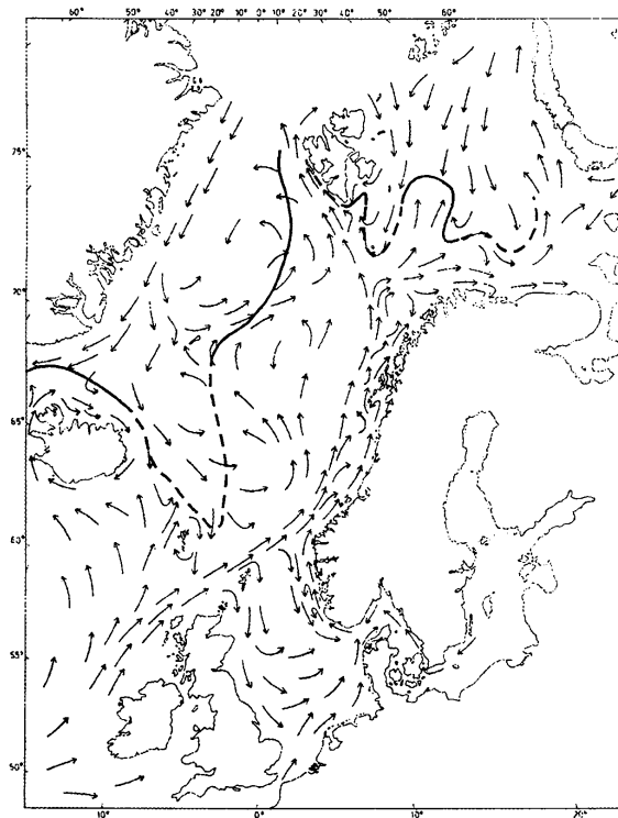
Figure 2 Main features of surface currents in the northeast Atlantic. The bold line indicates the mean position of the Arctic Frontal Zone (AFZ). The dotted line indicates where the position of the AFZ is most varying.
